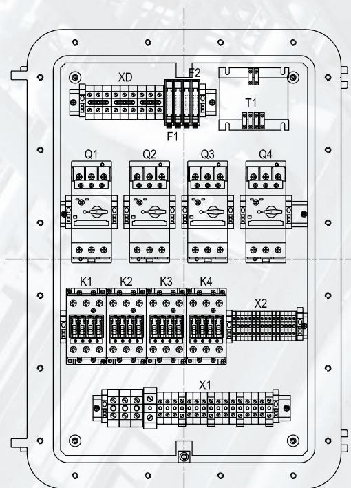
Internal layout
