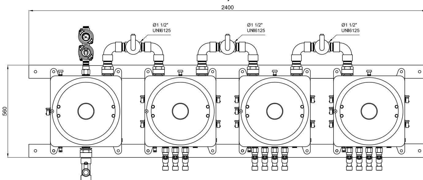
External layout
