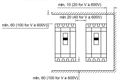
Minimum distances for 630/650A switches and contactors
