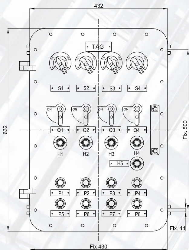
External layout
