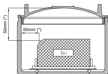
Example of interface unit without separator
