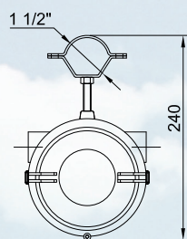
Mounting using 1.1/2" metal clamps TYPE "P"
