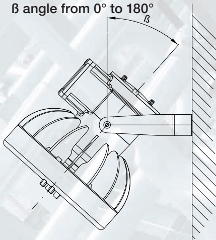
Example of wall mounting \beta angle from 0° to 180°
