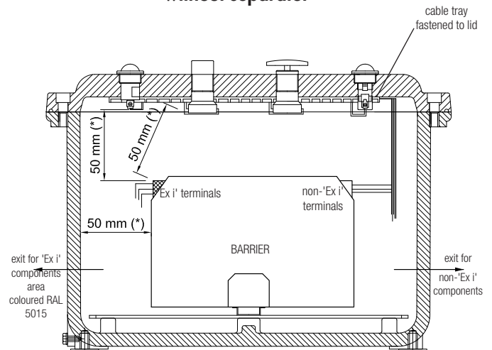
Example of interface unit without separator
